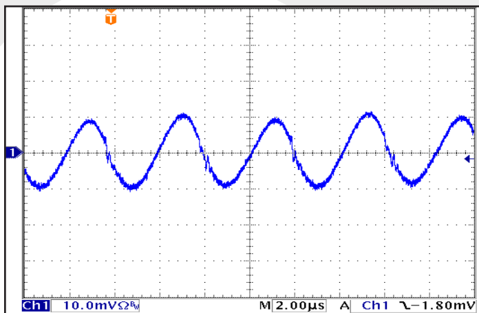
Figure 9: Input Terminal Current Ripple , i_C , at full rated output current and nominal input voltage with SynQor MCOTS filter module (200 mA/div). Bandwidth: 20 MHz. Timescale: 2.00μs/div. See Figure 13.
