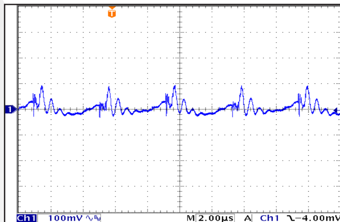
Figure 10: Output Voltage Ripple , V_{out} , at nominal input voltage and rated load current (100 mV/div). Load capacitance: 1 μF ceramic capacitor and 100 μF electrolytic capacitors. Bandwidth: 20 MHz. Timescale: 2.00μs/div. See Figure 13.
