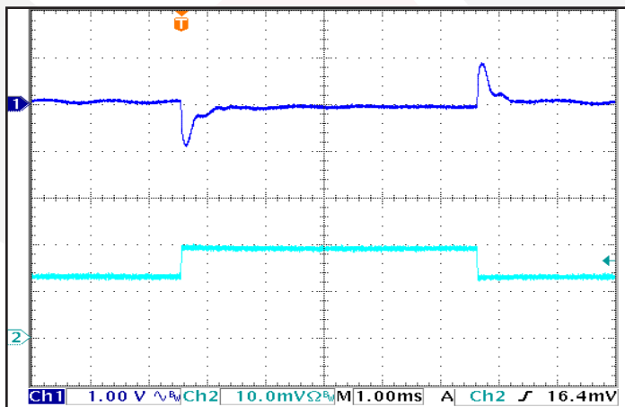
Figure 11: Output Voltage Response to Step-Change in Load Current , (50%-75%-50% of I_{out(max)} ; dI/dt = 5 A/μs). Load cap: 1 μF ceramic and 100 μF electrolytic capacitors. Ch 1: V_{out} (1 V/div); Ch 2: I_{out} (5 A/div). Timescale: 1.00ms/div.
